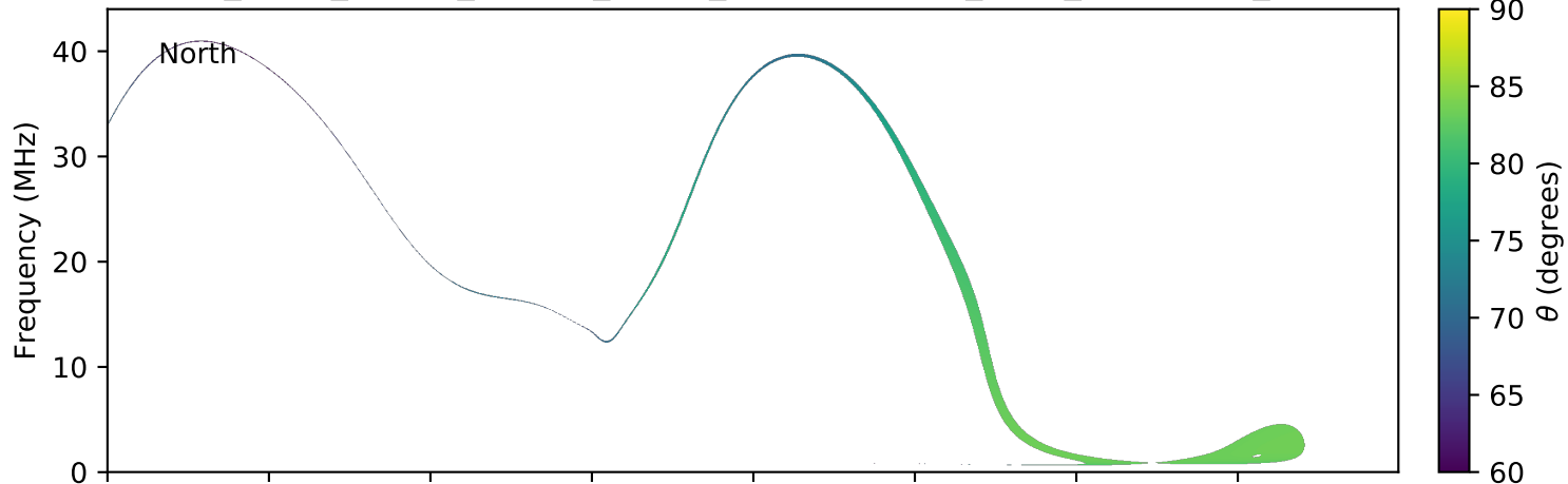
expres_earth_jupiter_europa_jrm09_lossc-wid1deg_3kev_20191108_v01.cdf
