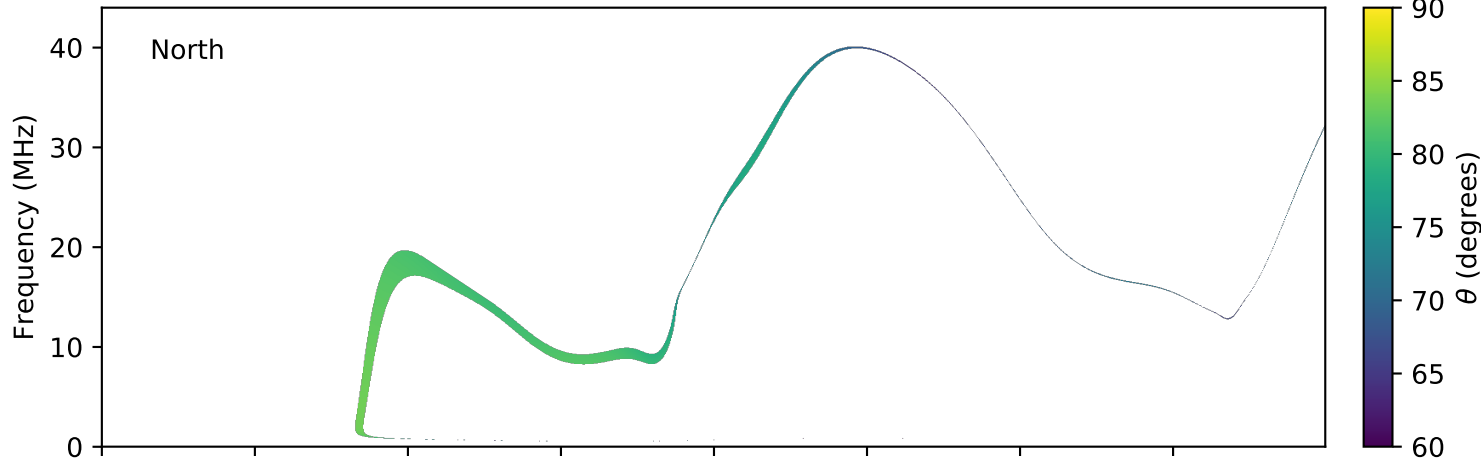
expres_earth_jupiter_europa_jrm09_lossc-wid1deg_3kev_20191107_v01.cdf
