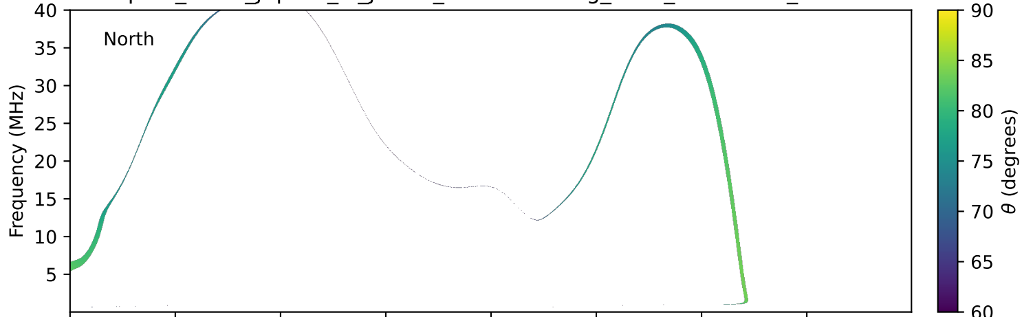
expres_earth_jupiter_io_jrm33_lossc-wid1deg_3kev_20191026_v11.cdf
