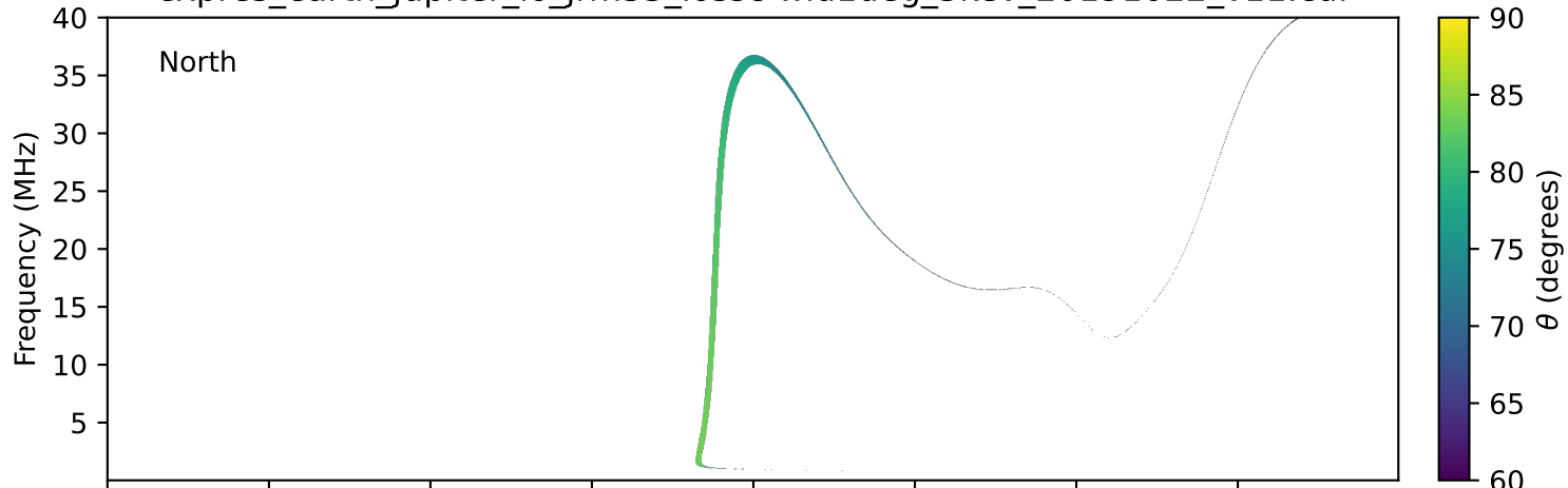
expres_earth_jupiter_io_jrm33_lossc-wid1deg_3kev_20191022_v11.cdf
