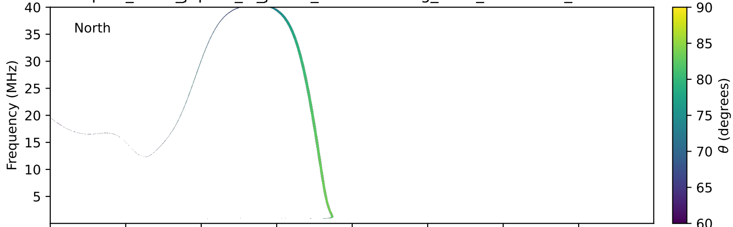
expres_earth_jupiter_io_jrm33_lossc-wid1deg_3kev_20191021_v11.cdf
