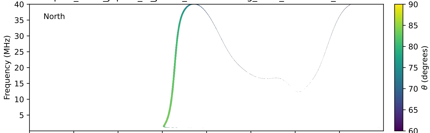
expres_earth_jupiter_io_jrm33_lossc-wid1deg_3kev_20191015_v11.cdf
