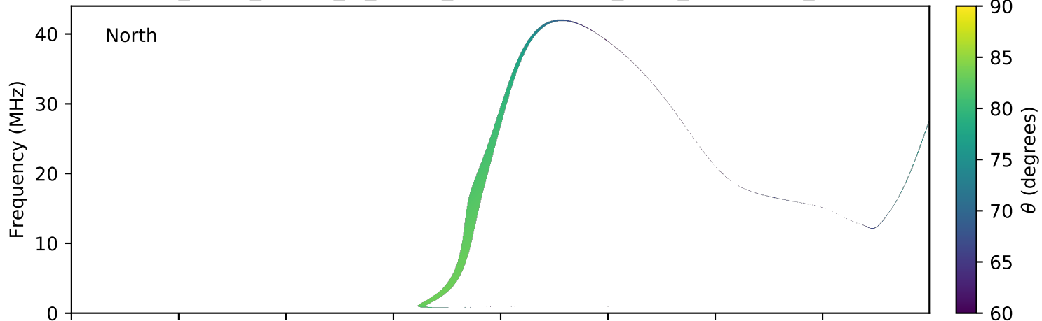
expres_earth_jupiter_io_jrm09_lossc-wid1deg_3kev_20191031_v01.cdf
