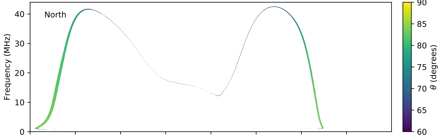
expres_earth_jupiter_io_jrm09_lossc-wid1deg_3kev_20191019_v01.cdf
