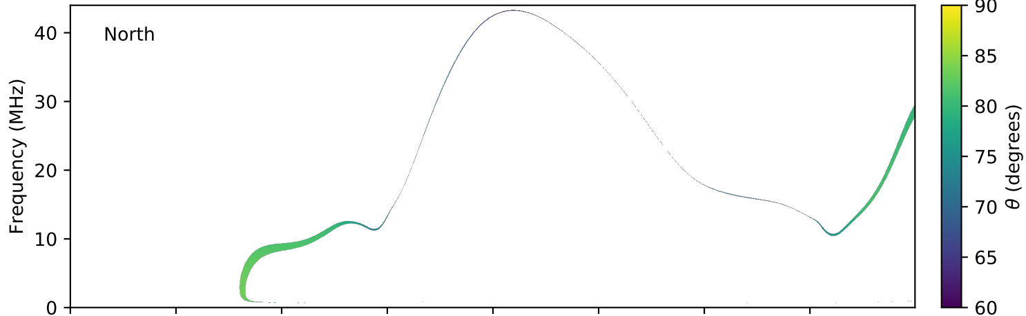
expres_earth_jupiter_io_jrm09_lossc-wid1deg_3kev_20191017_v01.cdf
