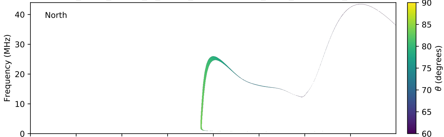
expres_earth_jupiter_io_jrm09_lossc-wid1deg_3kev_20191015_v01.cdf
