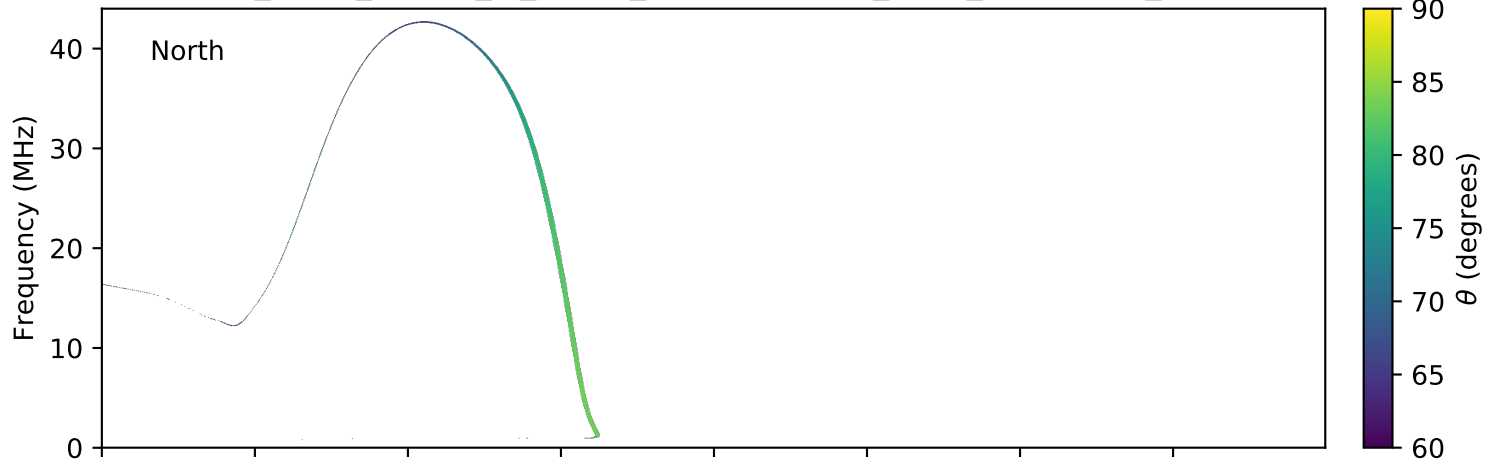
expres_earth_jupiter_io_jrm09_lossc-wid1deg_3kev_20191007_v01.cdf
