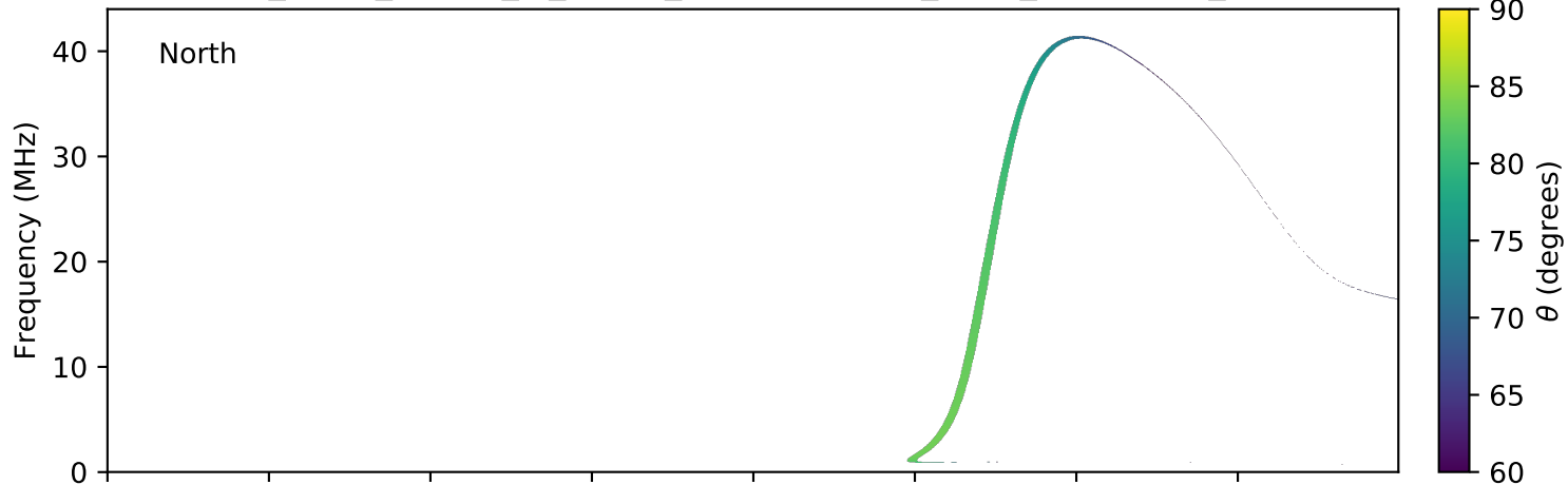
expres_earth_jupiter_io_jrm09_lossc-wid1deg_3kev_20191006_v01.cdf
