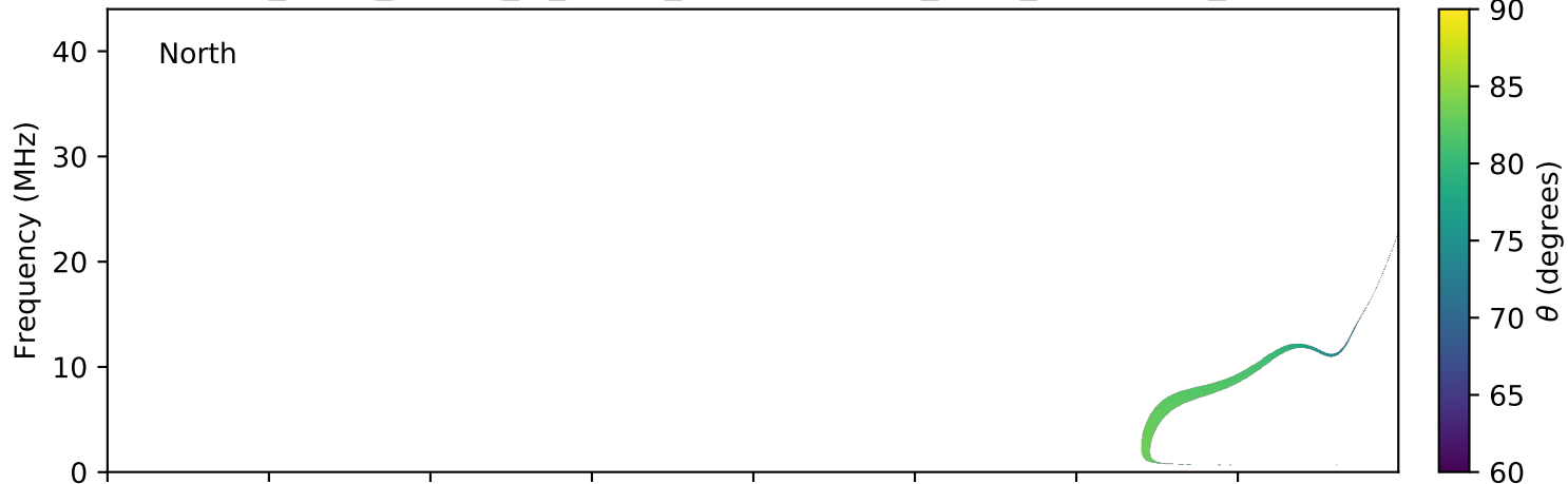
expres_earth_jupiter_io_jrm09_lossc-wid1deg_3kev_20191004_v01.cdf
