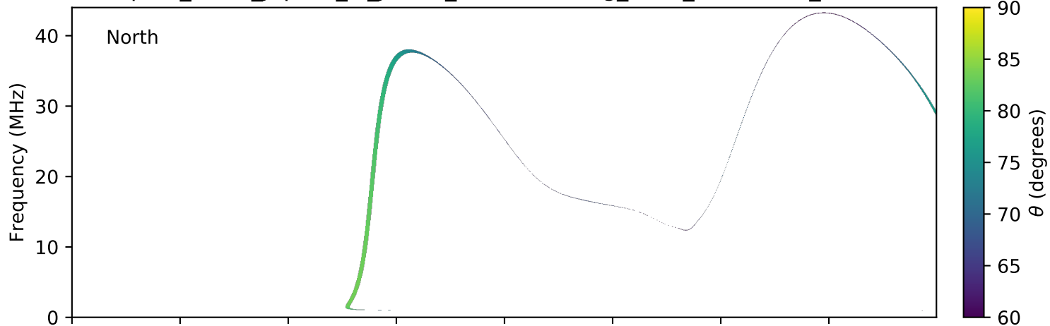
expres_earth_jupiter_io_jrm09_lossc-wid1deg_3kev_20191001_v01.cdf
