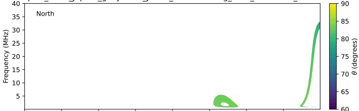
expres_earth_jupiter_ganymede_jrm33_lossc-wid1deg_3kev_20191031_v11.cdf
