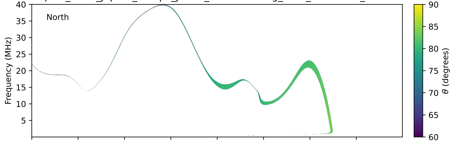
expres_earth_jupiter_europa_jrm33_lossc-wid1deg_3kev_20191021_v11.cdf
