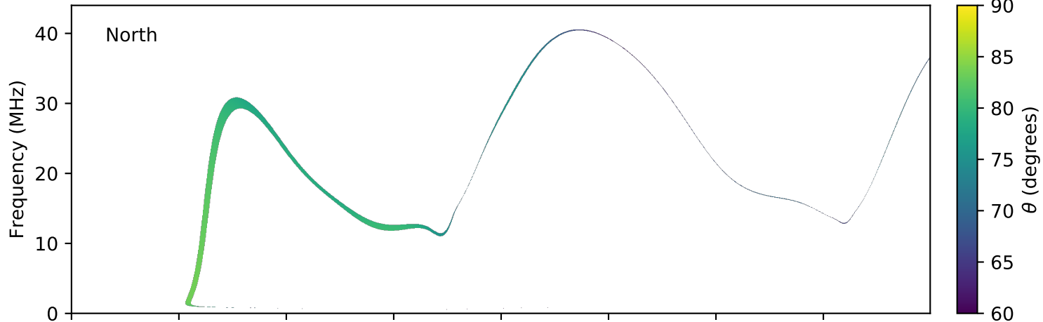
expres_earth_jupiter_europa_jrm09_lossc-wid1deg_3kev_20191031_v01.cdf
