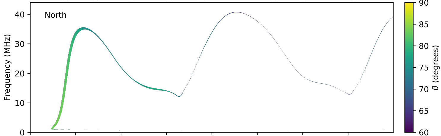
expres_earth_jupiter_europa_jrm09_lossc-wid1deg_3kev_20191024_v01.cdf
