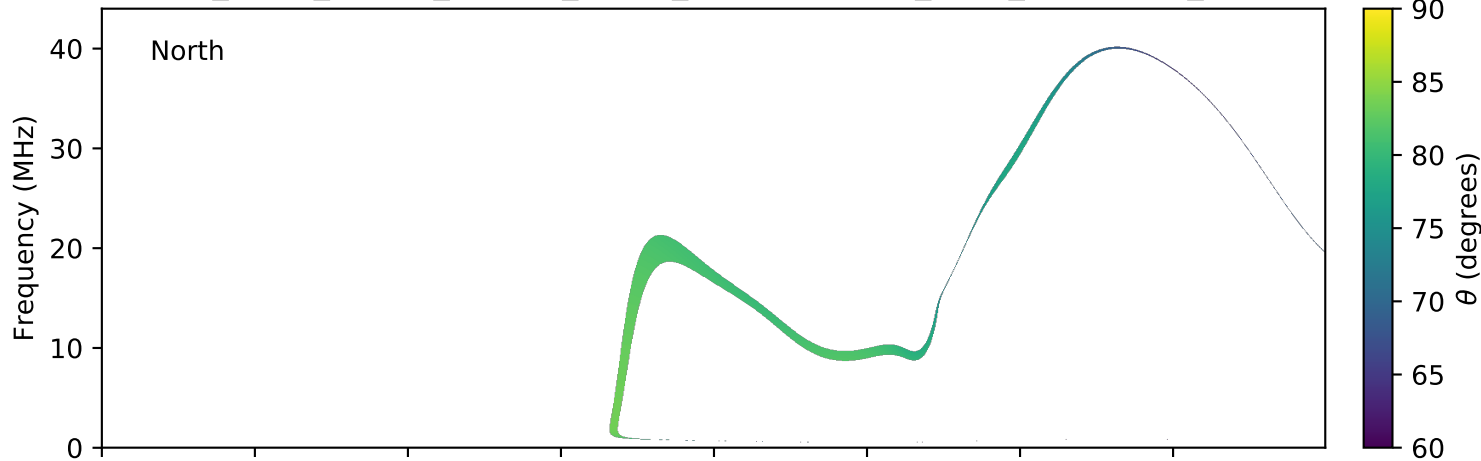
expres_earth_jupiter_europa_jrm09_lossc-wid1deg_3kev_20191020_v01.cdf
