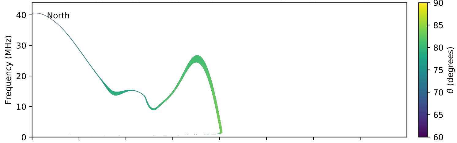
expres_earth_jupiter_europa_jrm09_lossc-wid1deg_3kev_20191018_v01.cdf
