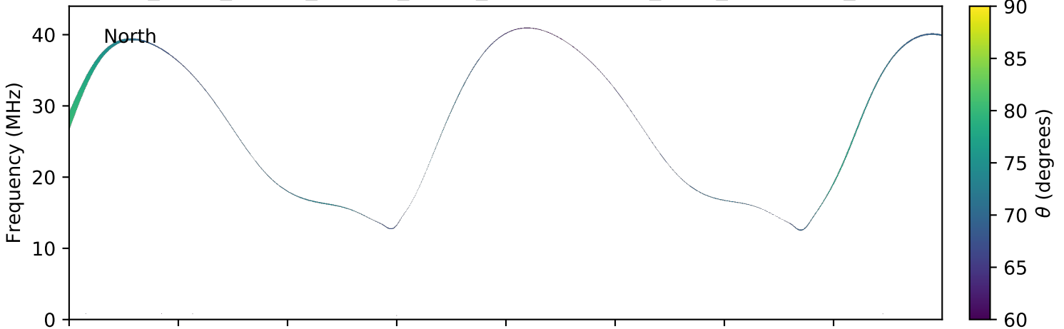
expres_earth_jupiter_europa_jrm09_lossc-wid1deg_3kev_20191010_v01.cdf
