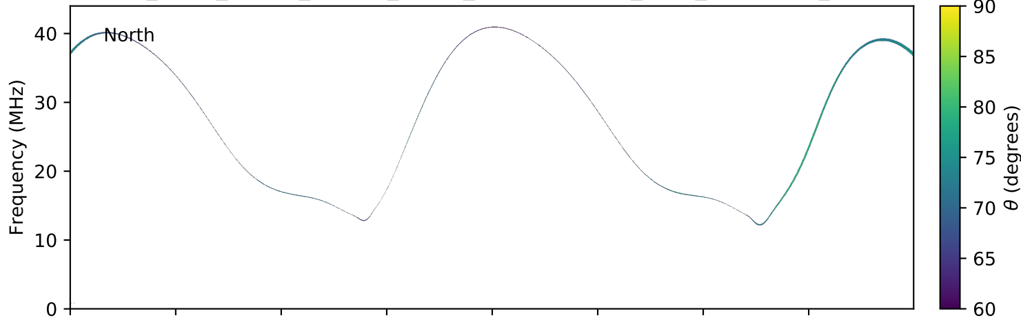
expres_earth_jupiter_europa_jrm09_lossc-wid1deg_3kev_20191003_v01.cdf
