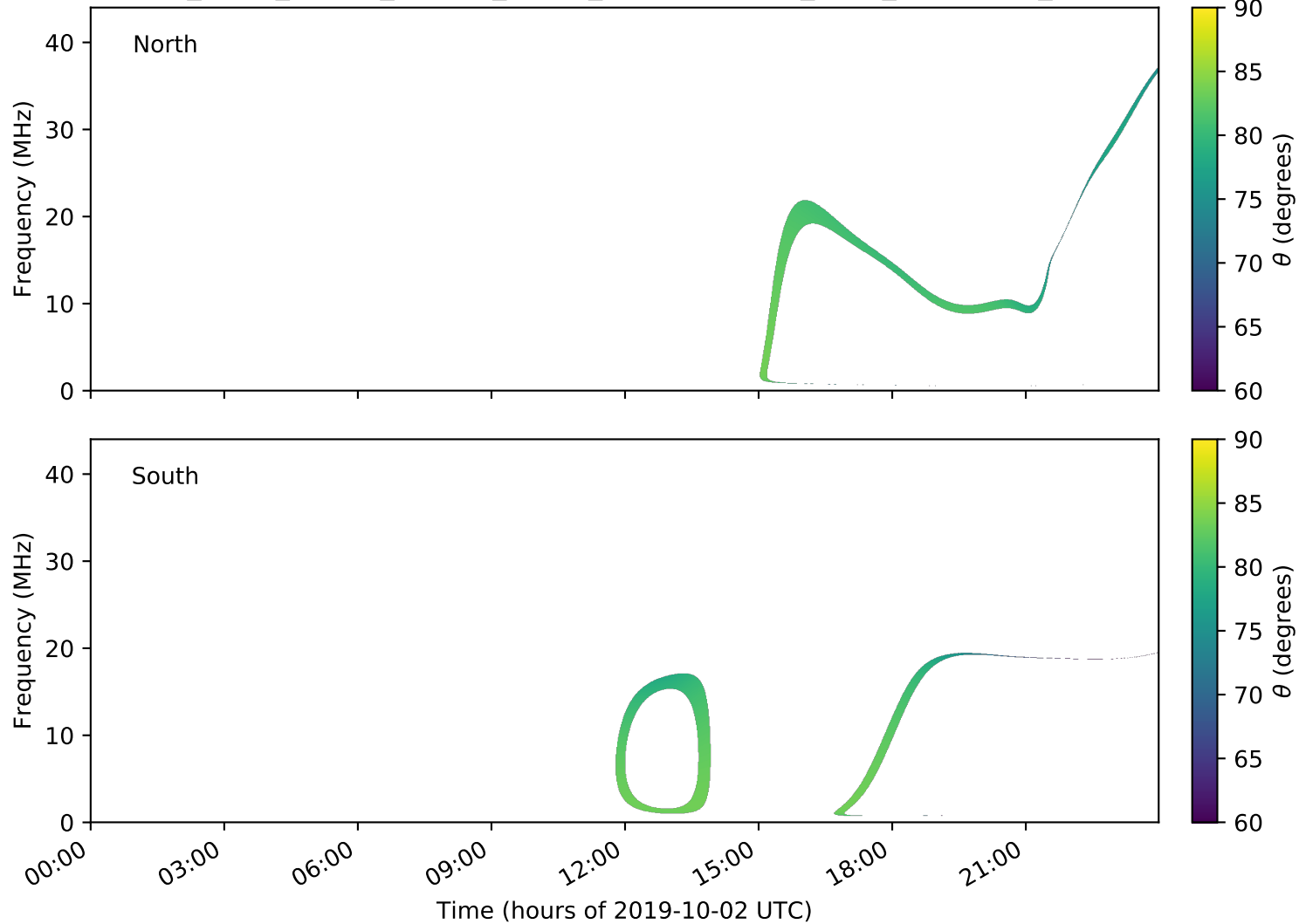
expres_earth_jupiter_europa_jrm09_lossc-wid1deg_3kev_20191002_v01.cdf
