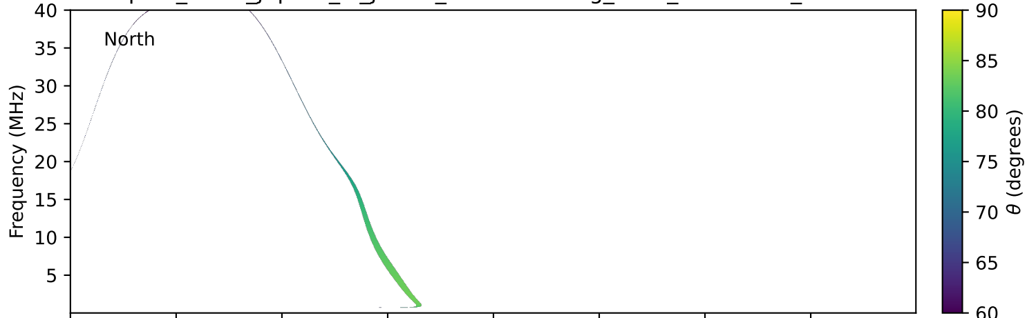
expres_earth_jupiter_io_jrm33_lossc-wid1deg_3kev_20190928_v11.cdf
