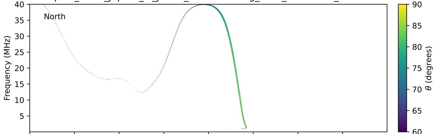
expres_earth_jupiter_io_jrm33_lossc-wid1deg_3kev_20190919_v11.cdf
