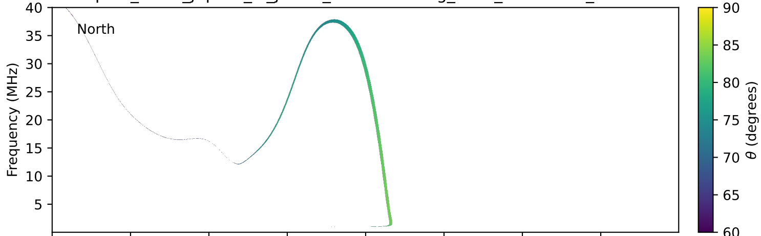
expres_earth_jupiter_io_jrm33_lossc-wid1deg_3kev_20190912_v11.cdf
