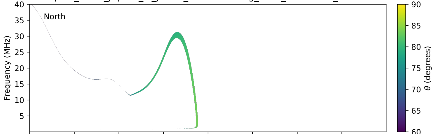
expres_earth_jupiter_io_jrm33_lossc-wid1deg_3kev_20190905_v11.cdf
