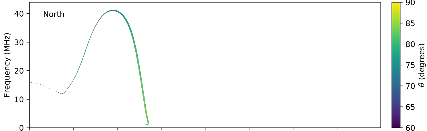
expres_earth_jupiter_io_jrm09_lossc-wid1deg_3kev_20190930_v01.cdf
