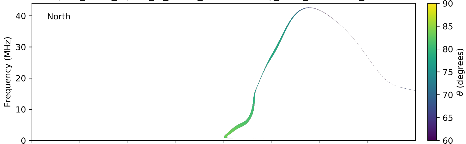
expres_earth_jupiter_io_jrm09_lossc-wid1deg_3kev_20190929_v01.cdf
