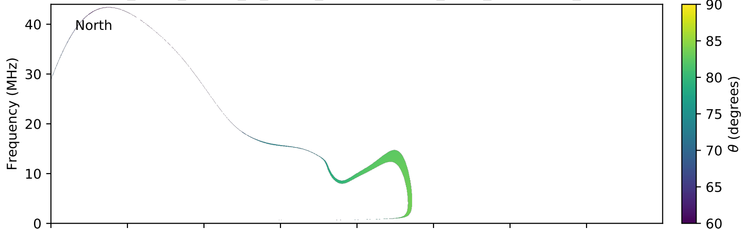
expres_earth_jupiter_io_jrm09_lossc-wid1deg_3kev_20190928_v01.cdf
