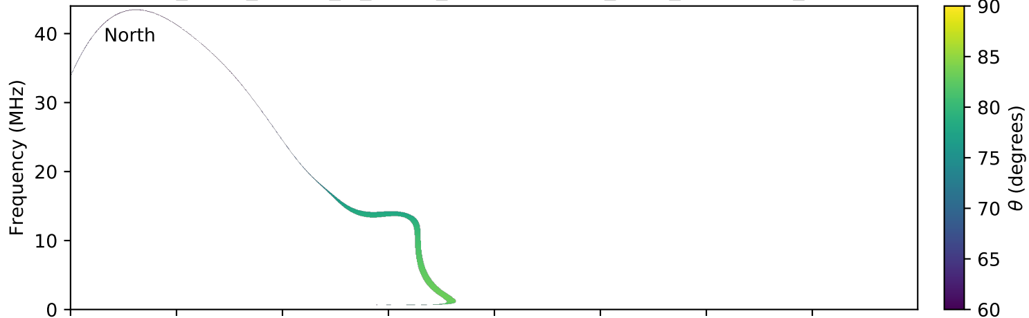
expres_earth_jupiter_io_jrm09_lossc-wid1deg_3kev_20190921_v01.cdf
