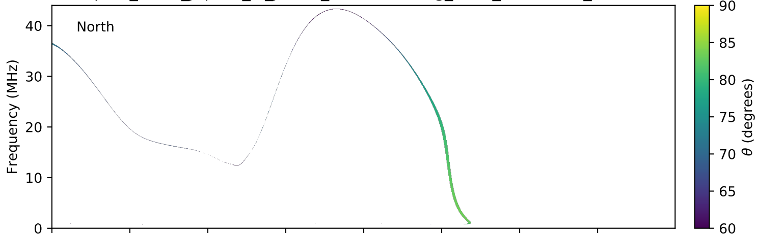
expres_earth_jupiter_io_jrm09_lossc-wid1deg_3kev_20190919_v01.cdf
