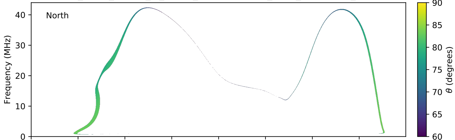
expres_earth_jupiter_io_jrm09_lossc-wid1deg_3kev_20190917_v01.cdf
