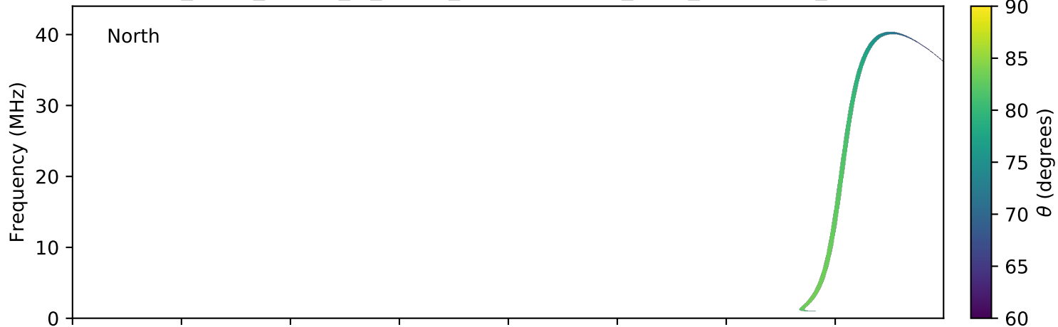
expres_earth_jupiter_io_jrm09_lossc-wid1deg_3kev_20190911_v01.cdf
