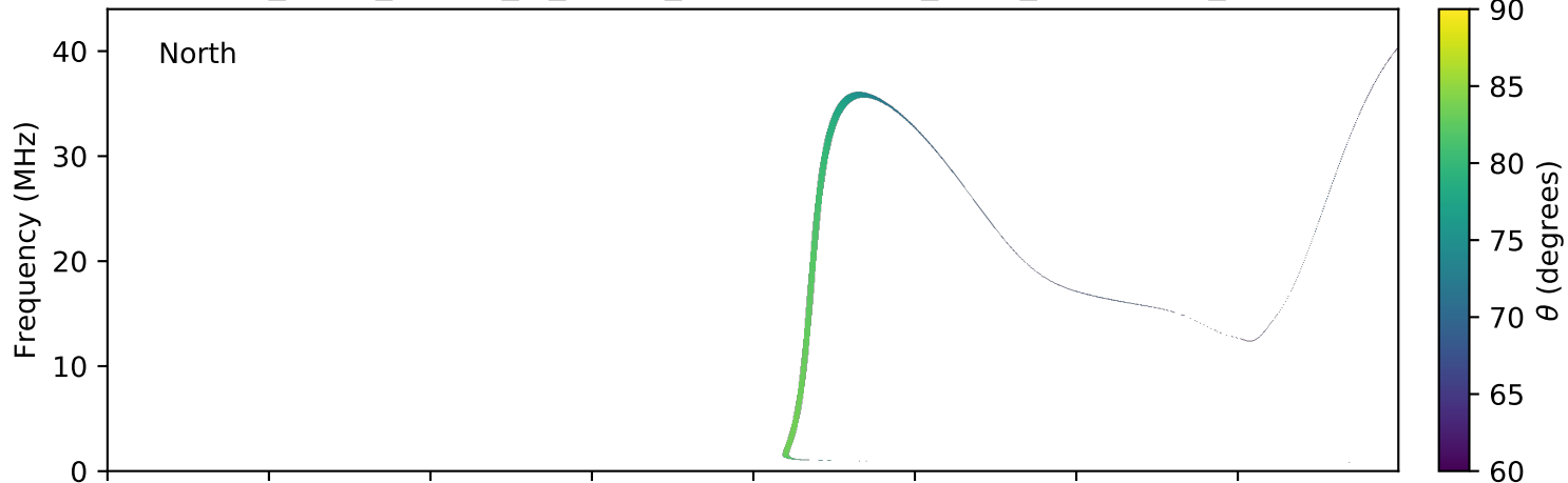
expres_earth_jupiter_io_jrm09_lossc-wid1deg_3kev_20190906_v01.cdf
