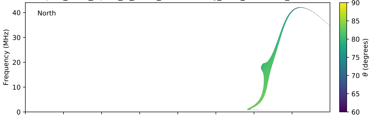
expres_earth_jupiter_io_jrm09_lossc-wid1deg_3kev_20190904_v01.cdf
