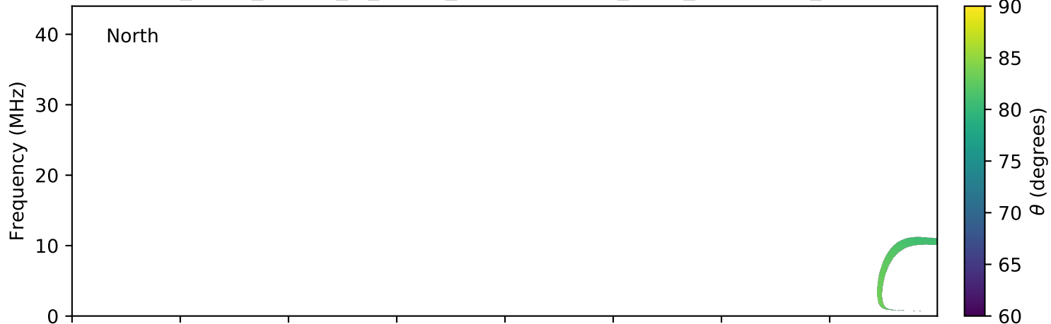
expres_earth_jupiter_io_jrm09_lossc-wid1deg_3kev_20190902_v01.cdf
