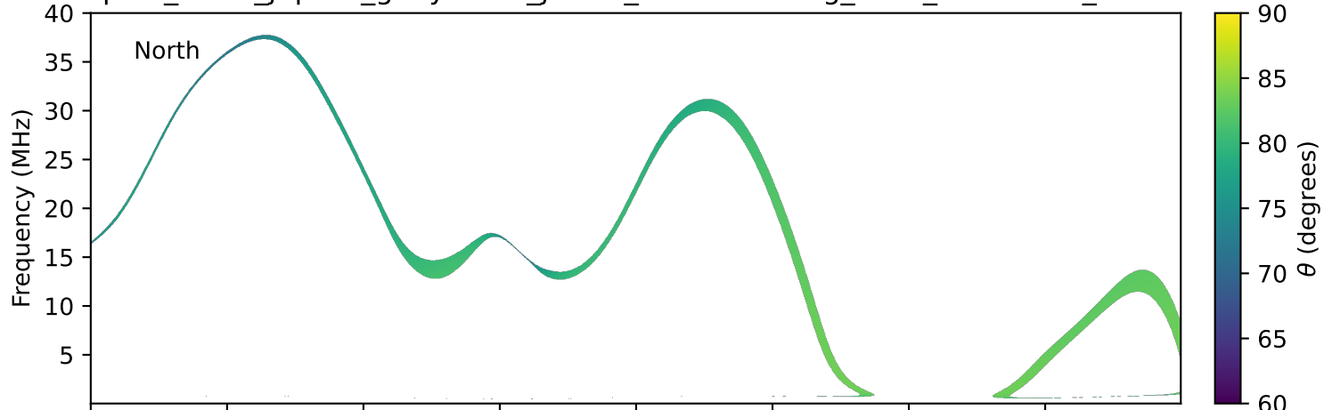
expres_earth_jupiter_ganymede_jrm33_lossc-wid1deg_3kev_20190921_v11.cdf
