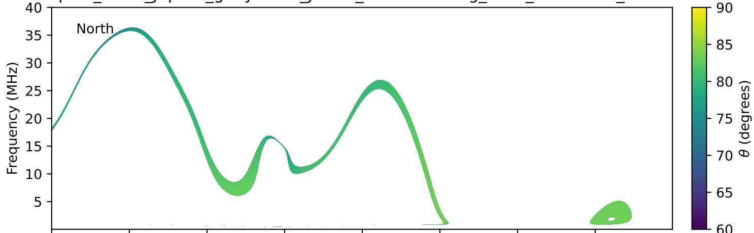
expres_earth_jupiter_ganymede_jrm33_lossc-wid1deg_3kev_20190914_v11.cdf
