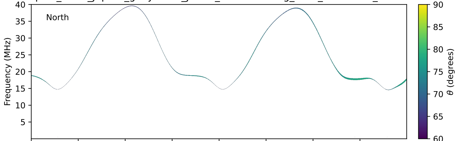
expres_earth_jupiter_ganymede_jrm33_lossc-wid1deg_3kev_20190913_v11.cdf
