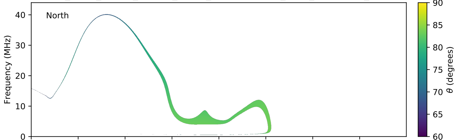
expres_earth_jupiter_europa_jrm09_lossc-wid1deg_3kev_20190923_v01.cdf
