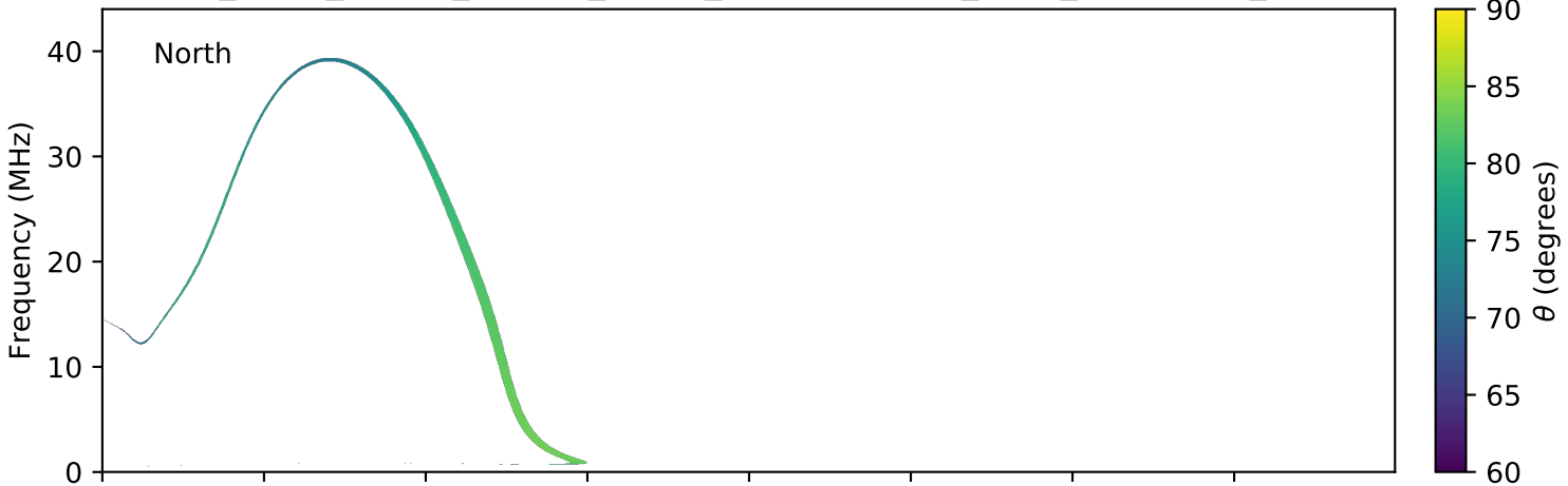
expres_earth_jupiter_europa_jrm09_lossc-wid1deg_3kev_20190916_v01.cdf
