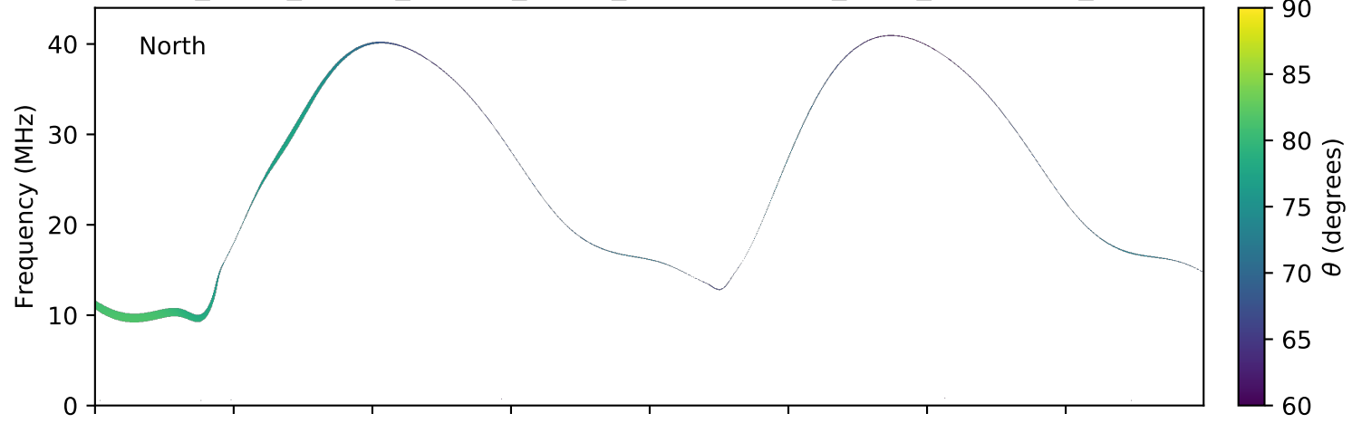
expres_earth_jupiter_europa_jrm09_lossc-wid1deg_3kev_20190915_v01.cdf
