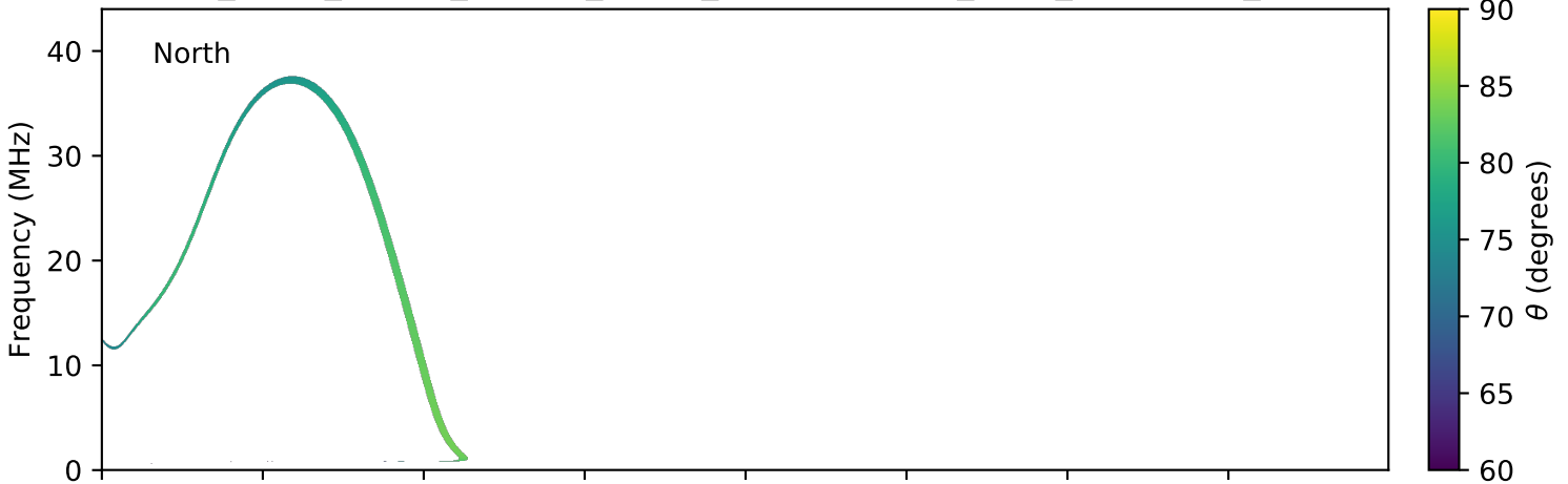
expres_earth_jupiter_europa_jrm09_lossc-wid1deg_3kev_20190909_v01.cdf
