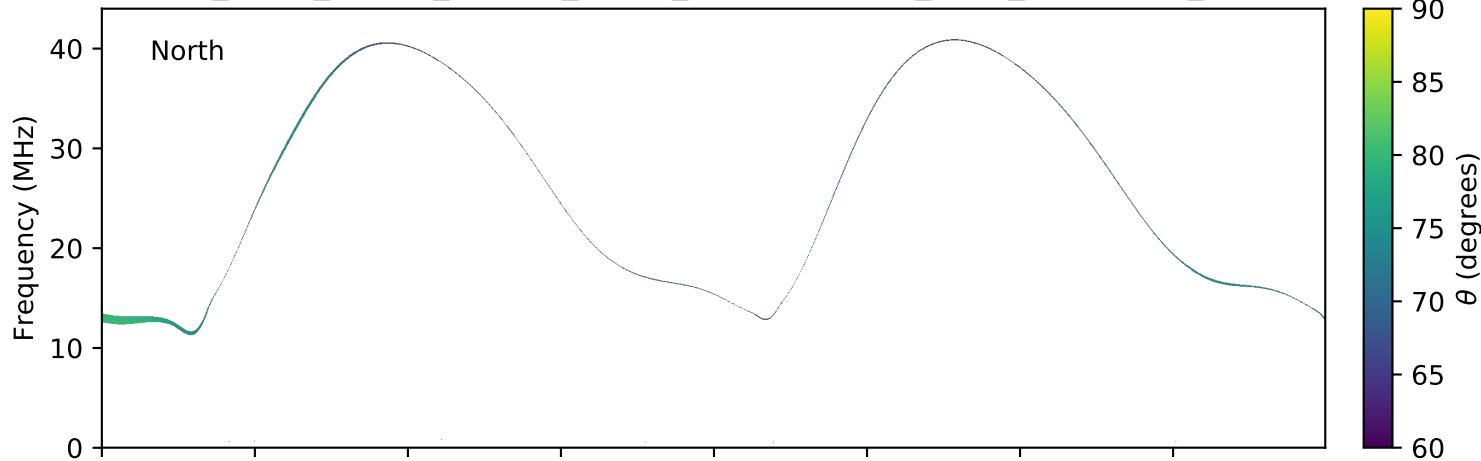
expres_earth_jupiter_europa_jrm09_lossc-wid1deg_3kev_20190908_v01.cdf
