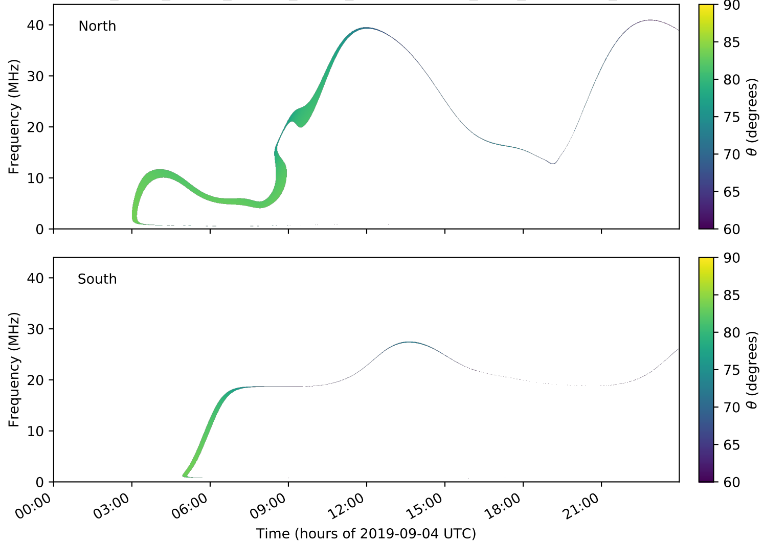
expres_earth_jupiter_europa_jrm09_lossc-wid1deg_3kev_20190904_v01.cdf
