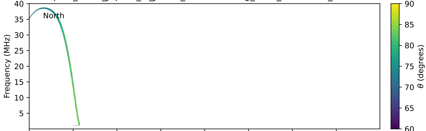
expres_earth_jupiter_io_jrm33_lossc-wid1deg_3kev_20190831_v11.cdf
