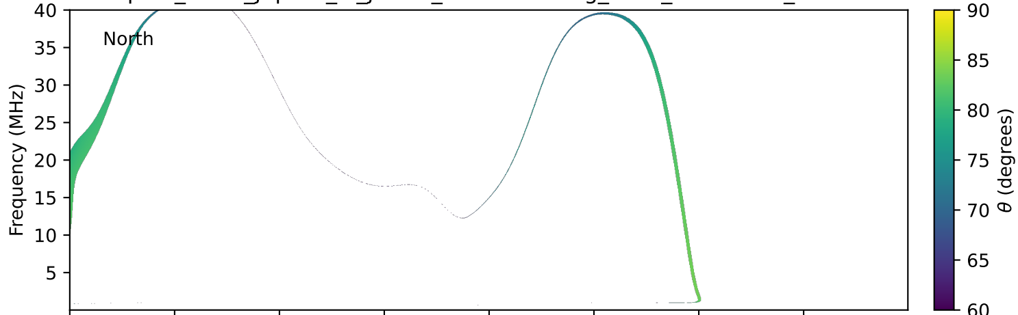
expres_earth_jupiter_io_jrm33_lossc-wid1deg_3kev_20190818_v11.cdf
