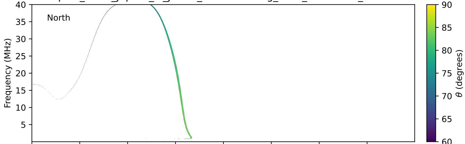
expres_earth_jupiter_io_jrm33_lossc-wid1deg_3kev_20190813_v11.cdf
