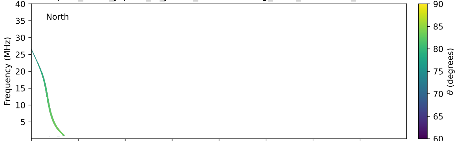
expres_earth_jupiter_io_jrm33_lossc-wid1deg_3kev_20190808_v11.cdf
